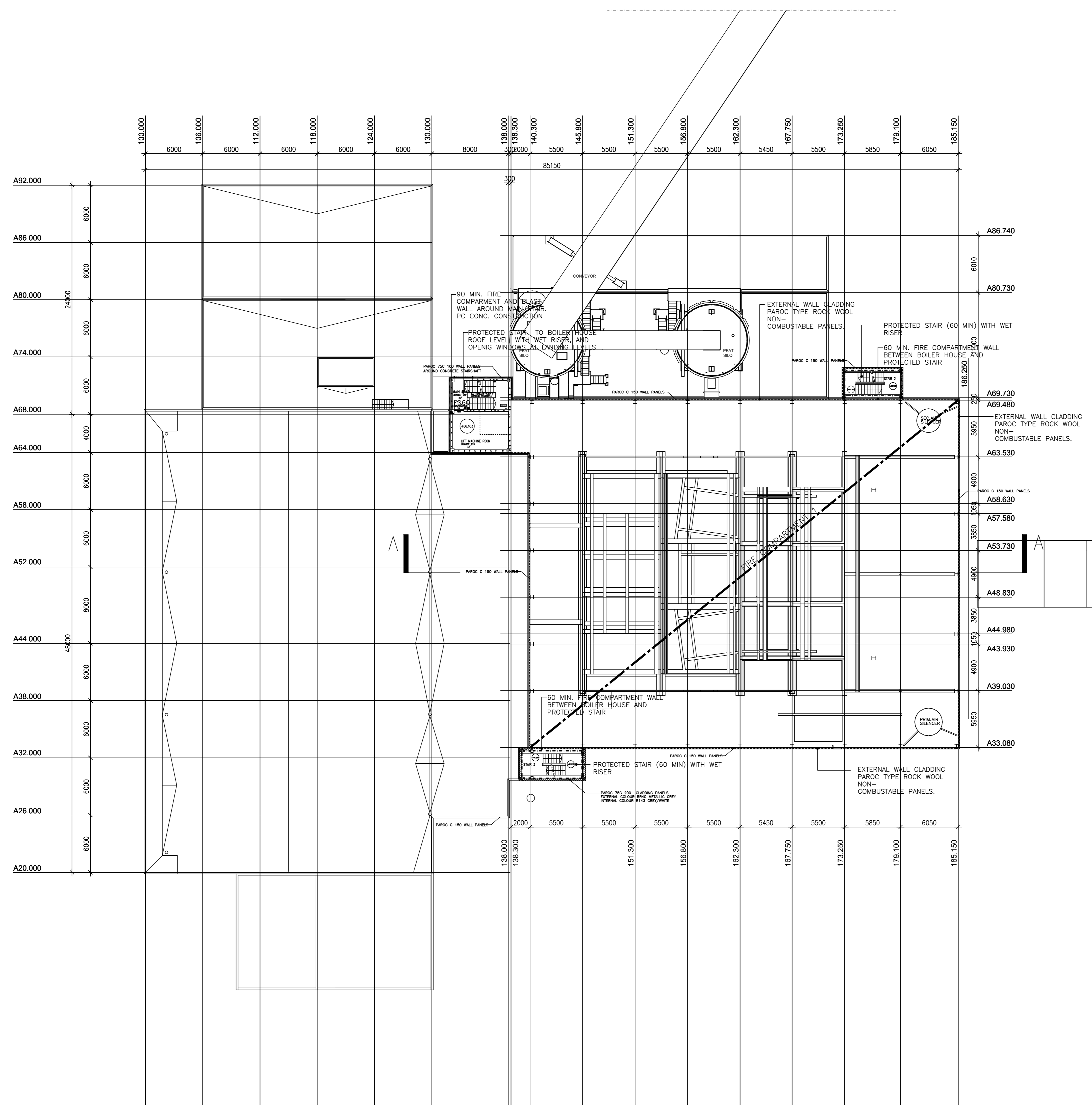
PLAN @ LEVEL +86.163m
